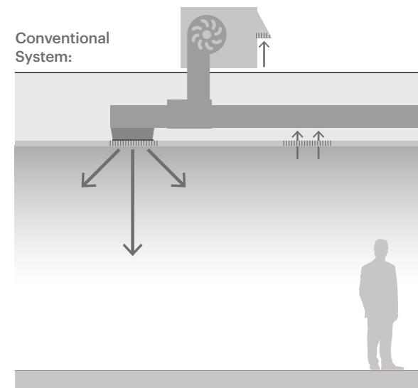
Overhead systems may require more fan energy to overcome static losses of generating the mixing, airflow patterns required within the space.
